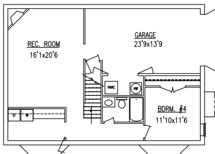
BASEMENT PLAN
